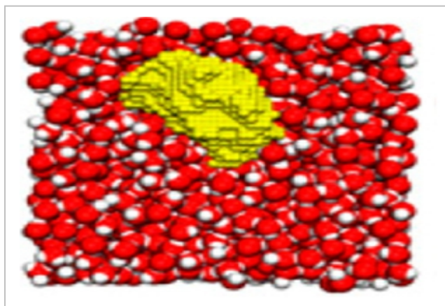
Critical cavitation bubble in water at -150 MPa from molecular dynamics simulations [3]
