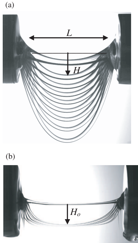
Fig. 1: Evolution of viscous threads hanging between two walls. The threads are obtained by squeezing a drop of silicone oil (viscosity \eta = 10 Pas) between the plates, which then are separated by a centimetric distance. (a) The initial thread length L and diameter D are 25 mm and 1.75 mm, respectively, and the interval \Delta t between two snapshots is 0.08 s. (b) L = 25 mm and D = 0.33 mm; \Delta t = 0.32 s. The thinnest thread adopts a U-shape, which basically stops at a small depth H_0 , contrasting with the catenary of the first series. It eventually breaks, which leads to two hanging disconnected pieces close to the walls.
